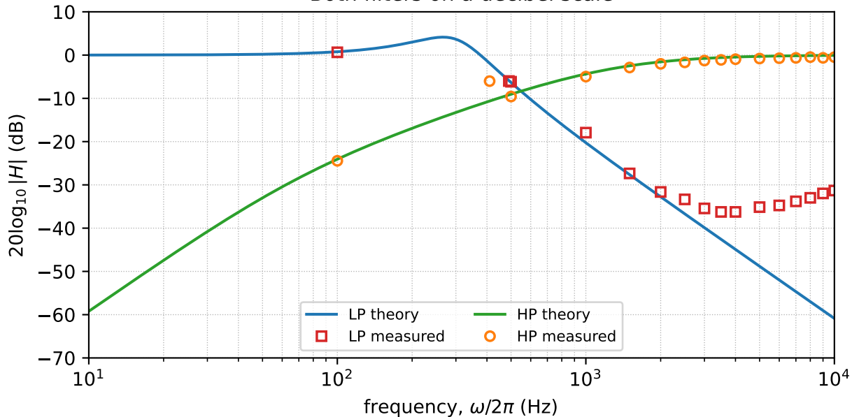
Both filters on a decibel scale
